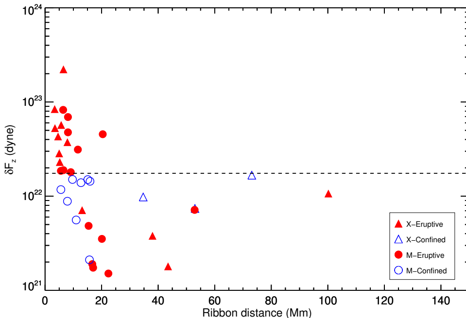
Figure 8. Scatter plot of vertical Lorentz force change vs ribbon distance. The values of Lorentz force change shown in the figure are estimated using the method based on the Lorentz force difference maps. Filled and empty symbols correspond to the eruptive and confined flares, respectively. The triangular and circular symbols imply X-class and M-class flares, respectively. The horizontal dashed line is drawn to illustrate the threshold value of change in Lorentz force. Few data points overlap each other.
