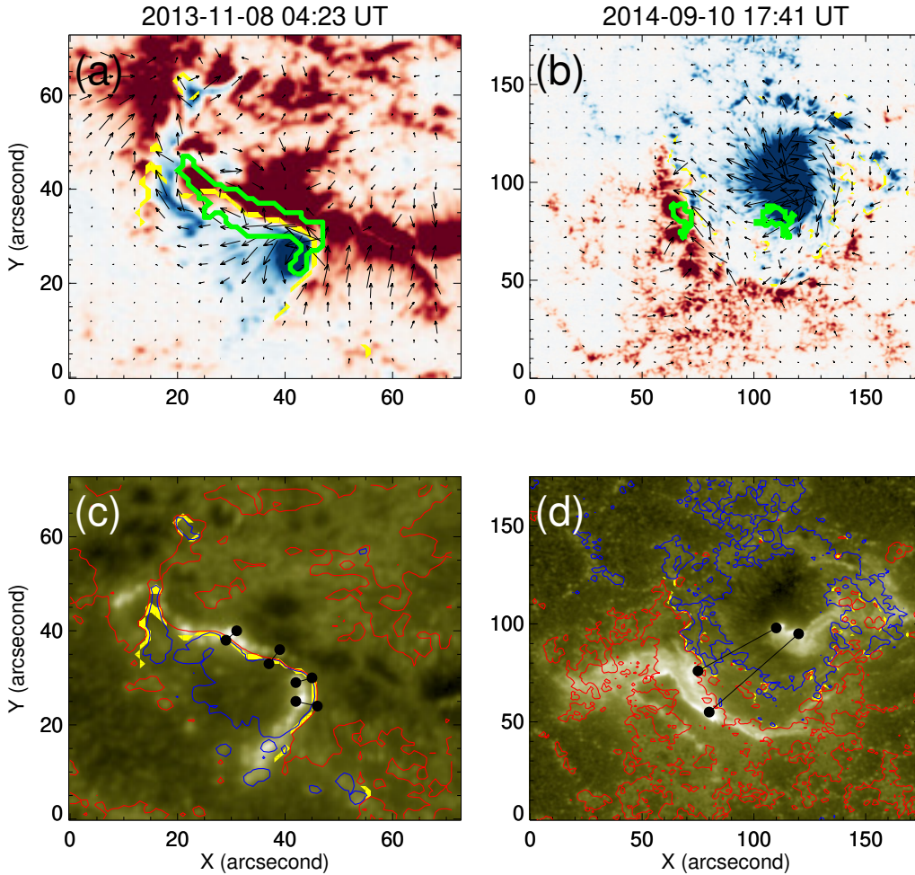
Figure 7. Illustrations demonstrating the calculation of ribbon distances for two events. Panels a and b represent the photospheric magnetic field maps for the two events occurred on 2013-11-08 04:23 UT and 2014-09-10 17:41 UT respectively. The red/blue colors represent the positive/negative polarities of B_r , plotted within a range of \pm 500 Gauss. The yellow line is indicative of the polarity inversion line (PIL) and the green contour signifies the region where the significant change in Lorentz force is observed.
