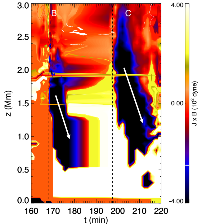
Figure 10. Height–time diagram of Lorentz force from the 3D MHD simulation to show its downward propagation. The dashed vertical lines represent the time of the two synthetic flares. The arrow is for guiding the eye towards the propagation direction of the Lorentz force.
