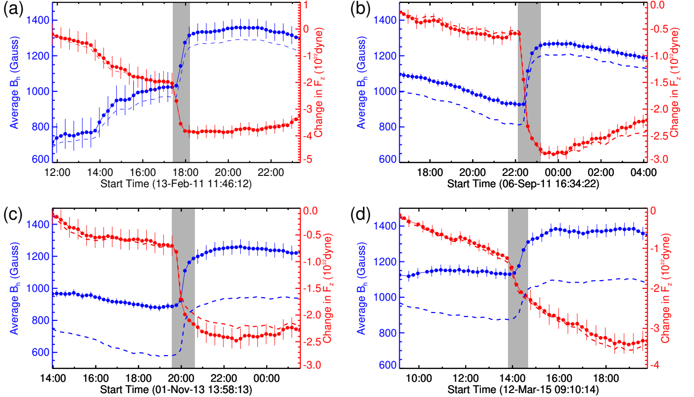
Figure 3. Temporal evolution of average horizontal magnetic fields (blue) and vertical Lorentz force (red) calculated by Lorentz force (solid) and horizontal magnetic field (dashed) contouring method. The panels a and b represent eruptive, whereas the panels c and d represent confined events. The shaded region corresponds to the duration of field change. The vertical error bars represents the fluctuations at a 3\sigma level in both pre- and post flare states.
