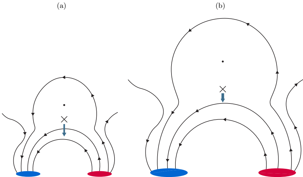
Figure 6. A sketch of the magnetic field configuration of (a) eruptive event with higher Lorentz force change and (b) eruptive event with lower Lorentz force change. Red and blue filled regions are positive and negative polarity regions whereas solid lines refer to the magnetic field lines. The X mark represents the location of the reconnection site and the downward arrow implies the direction of vertical Lorentz force responsible for the increase of horizontal magnetic field.
