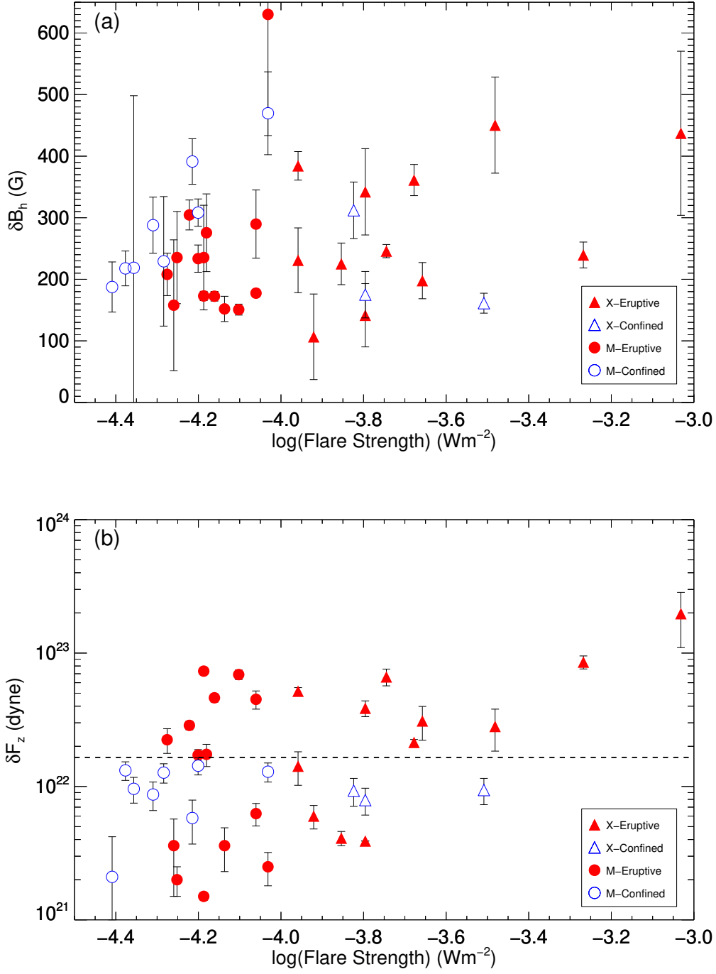
Figure 4. Scatter plot of (a) Average horizontal magnetic field change \delta B_h vs logarithmic flare strength and (b) Vertical Lorentz force change \delta F_z vs logarithmic flare strength for RoIs identified based on the difference maps of horizontal magnetic field. Filled and empty symbols correspond to the eruptive and confined flares, respectively. The triangular and circular symbols are for X-class and M-class flares, respectively. The horizontal dashed line indicates the threshold Lorentz force above which no confined flares are observed.
